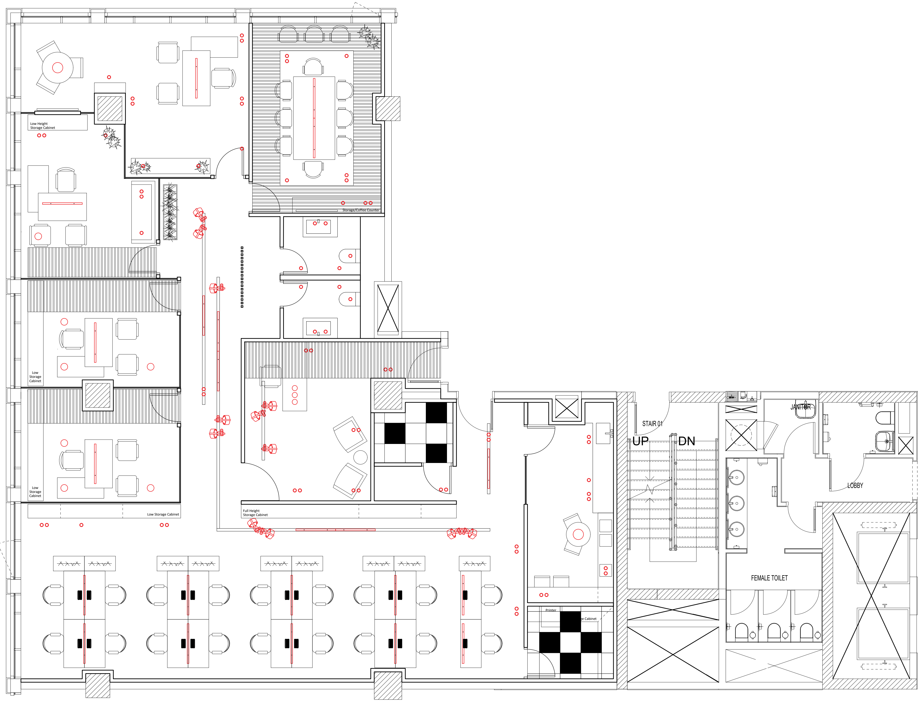
A 109 Reflected Ceiling Plan Second Floor
